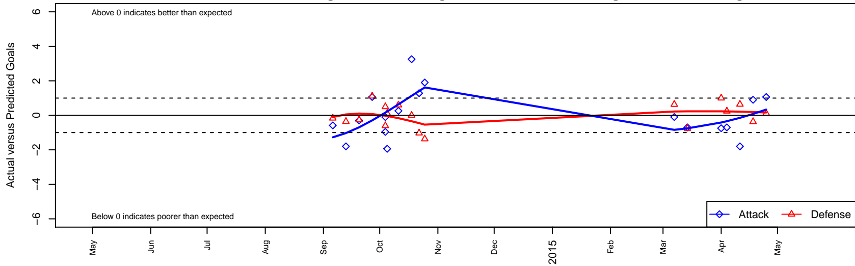
Neto United B00 Dots are actual minus expected GF (blue circles) and GA (red triangles). Blue line is smoothed change in attack strength. Red is smoothed change in defense strength.
